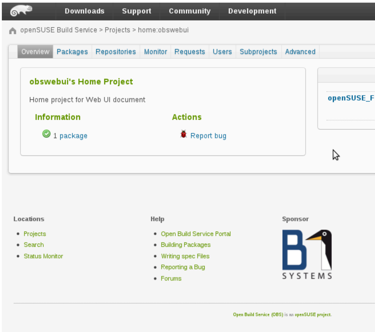
FIGURE 12.14: FLOOD_BUILD_SUCCESS
