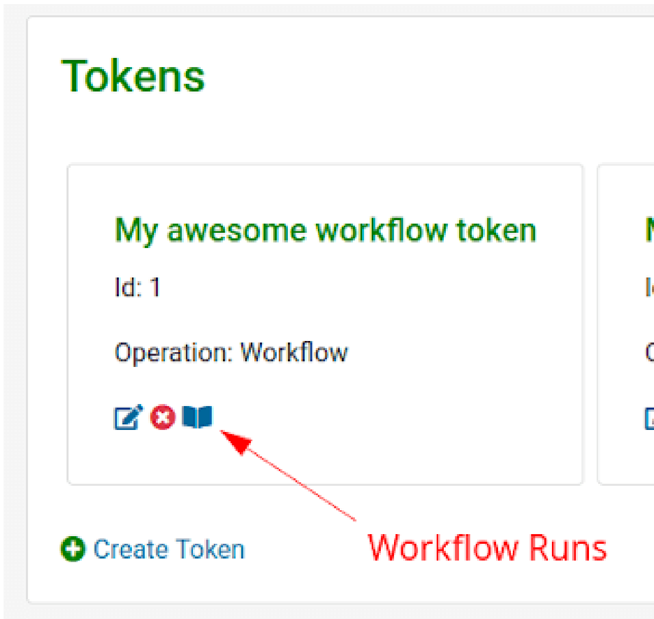
FIGURE 8.7: TOKENS LIST
