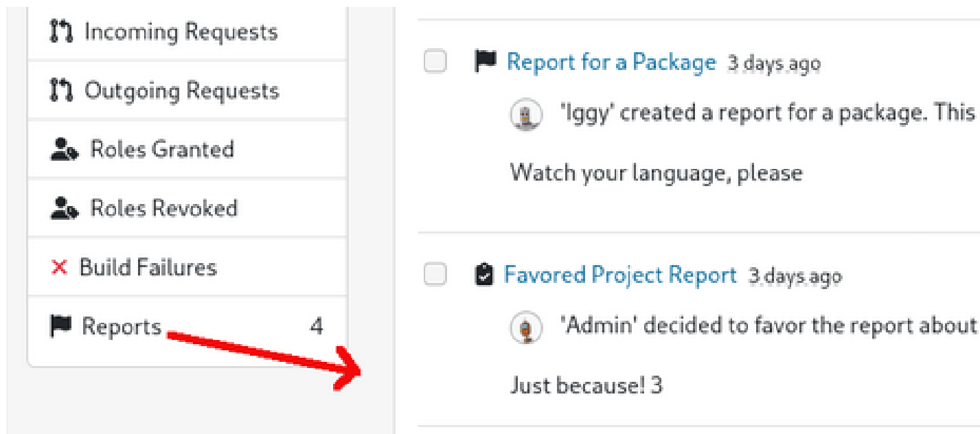
FIGURE 11.7: MODERATION-RELATED NOTIFICATIONS
