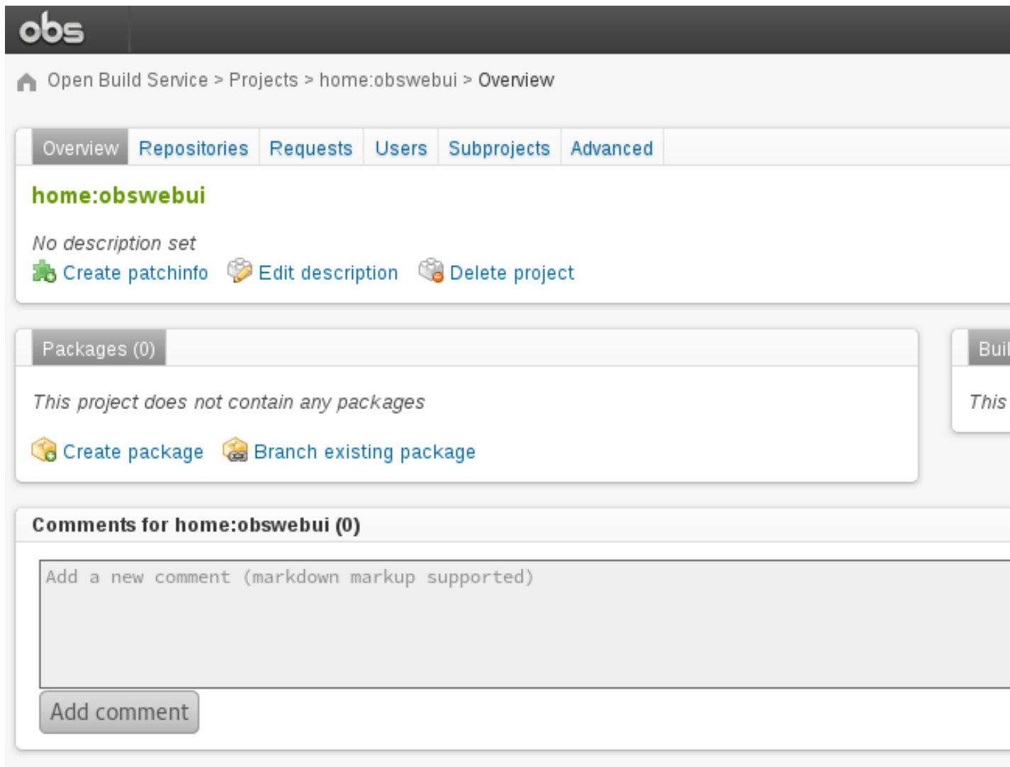
FIGURE 12.4: PROJECT PAGE
