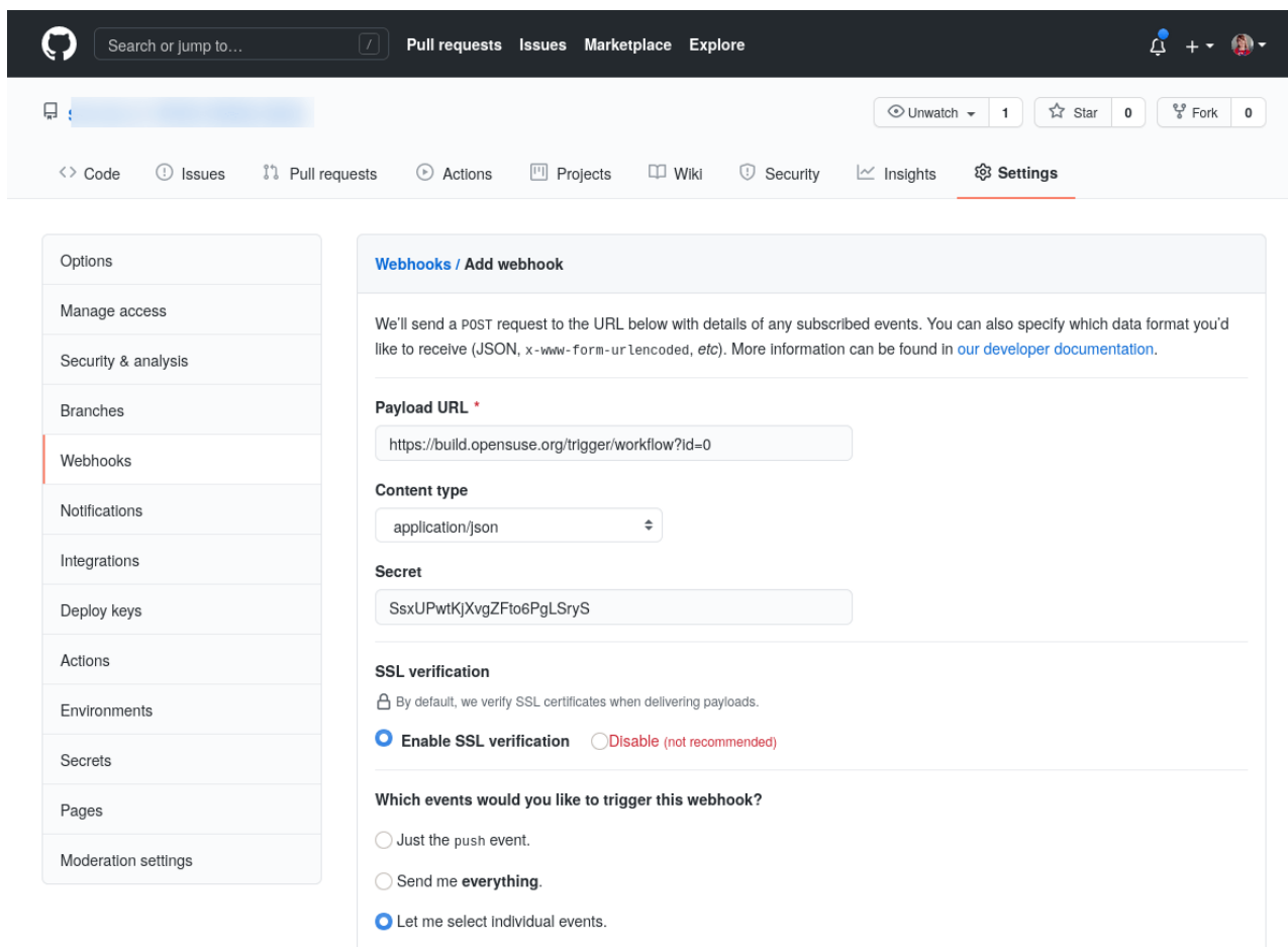
FIGURE 8.1: WEBHOOKS ON GITHUB.
