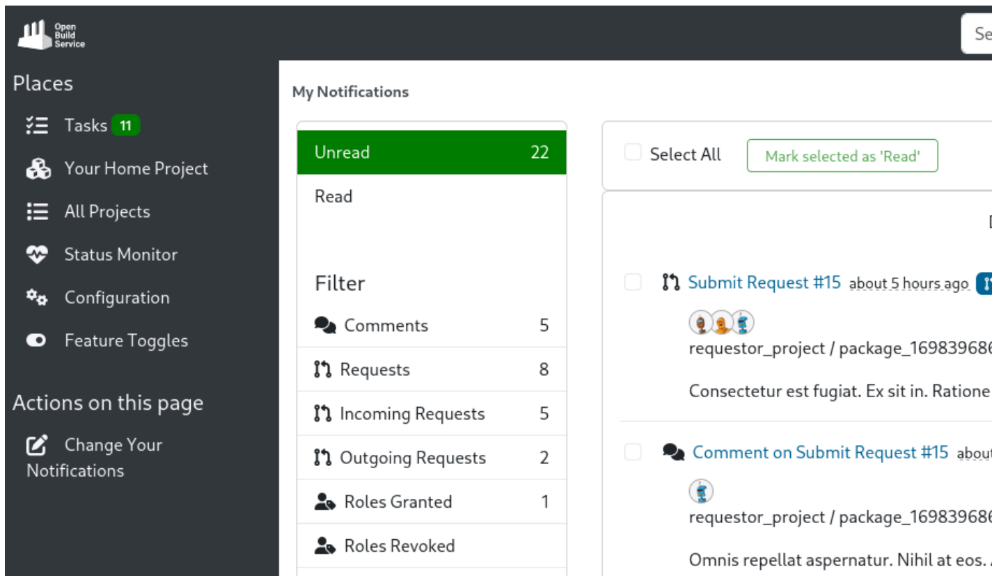
FIGURE 10.5: NOTIFICATIONS PAGE.
