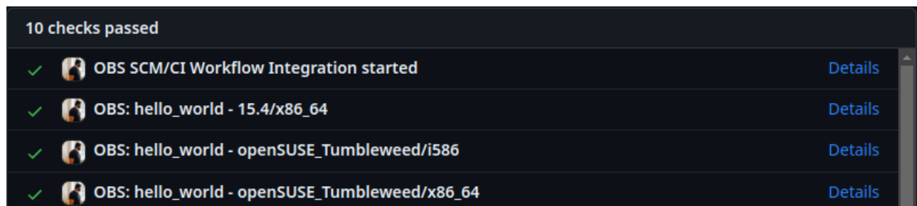
FIGURE 8.5: BUILD STATUS
